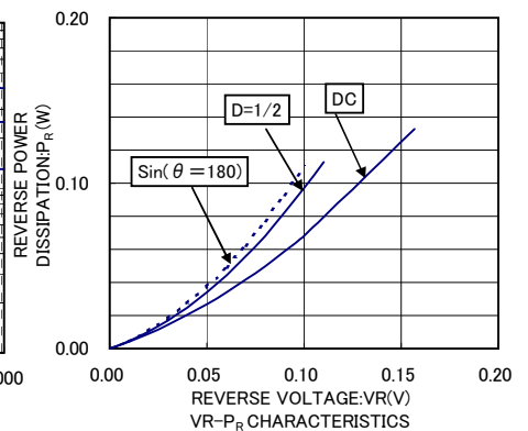
VR-Pr CHARACTERISTICS
