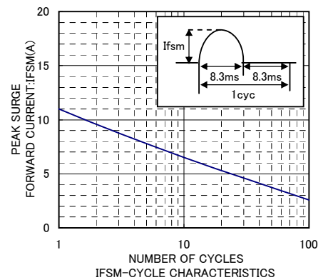
IFSM-CYCLE CHARACTERISTICS
