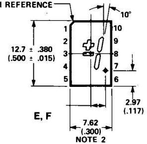
MITERED CORNER FOR PIN 1 REFERENCE
