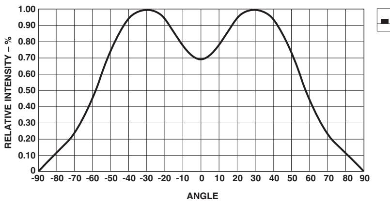
Figure 5. Relative intensity vs. angle for HSMx-C110.
