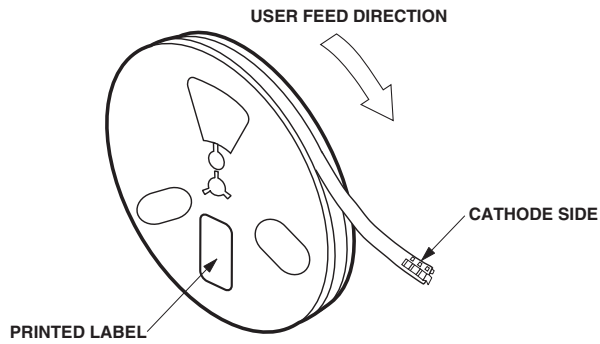
Figure 13. Reeling orientation.
