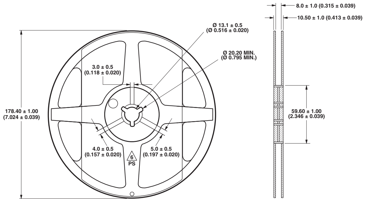
Figure 14. Reel dimensions.
