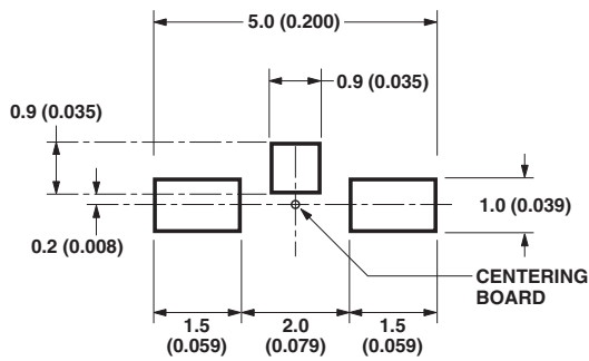
Figure 9. Recommended soldering pattern for HSMx-C110.
