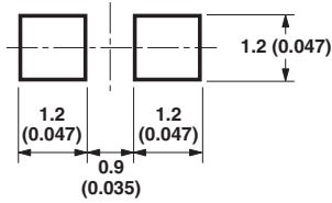
Figure 10. Recommended soldering pattern for HSMx-C170.
