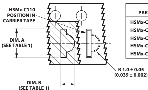
Figure 15. Tape dimensions.
