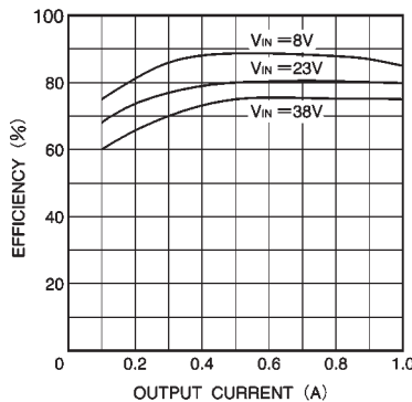
Fig.12 Efficiency
