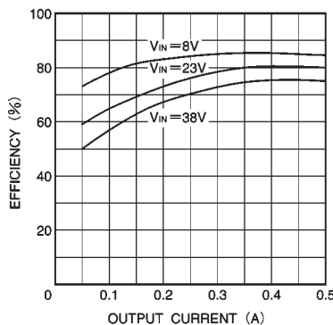
Fig.15 Efficiency
