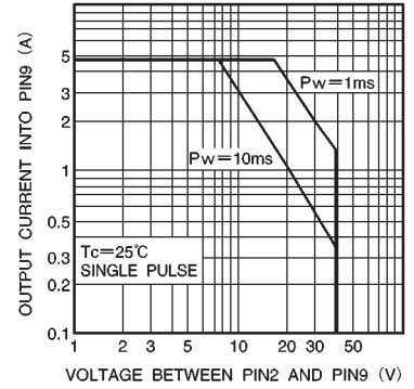
Fig. 19 Safe operation range (ASO)
