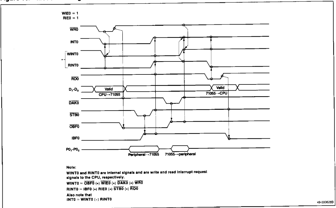
Figure 16. Mode 2 Timing
