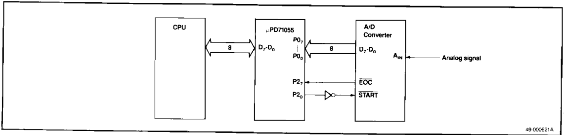
Figure 8. A/D Converter Example
