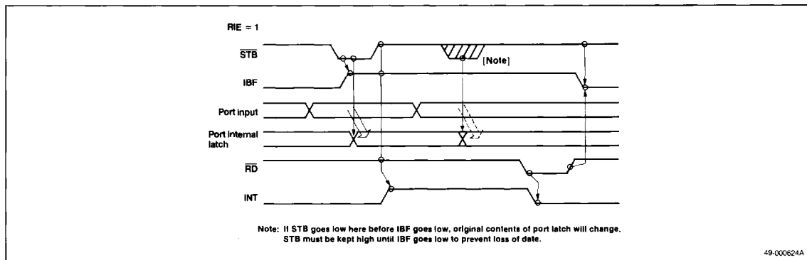
Figure 10. Mode 1 Input Timing
