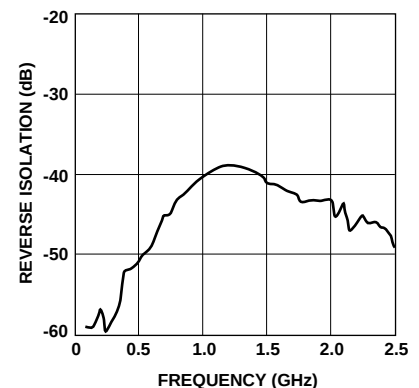
Figure 18. Measured Isolation.
