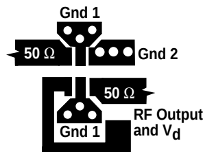
Figure 11. RF Layout
