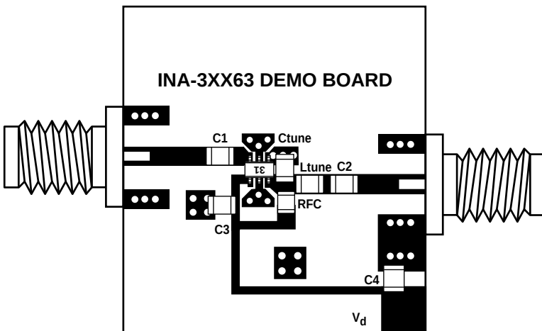
Figure 14. Assembled Amplifier.
