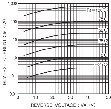
Fig.5 Reverse current vs. reverse voltage
