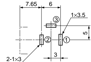
HOLE LAYOUT (BOTTOM VIEW)
