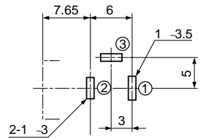
HOLE LAYOUT (BOTTOM VIEW)
