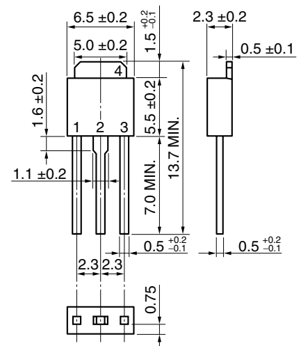
TO-251 (MP-3)
