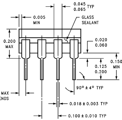
8-Pin Ceramic Dual-In-Line Package Order Number LM6181AMJ/883 NS Package Number J08A
