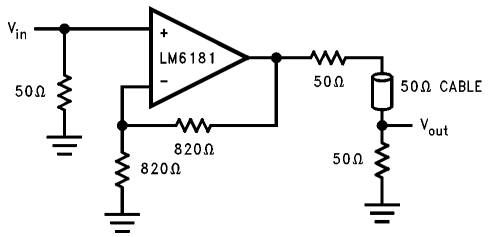
Cable Driver
