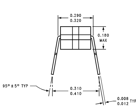
8-Pin Ceramic Dual-In-Line Package Order Number LM6181AMJ/883 NS Package Number J08A
