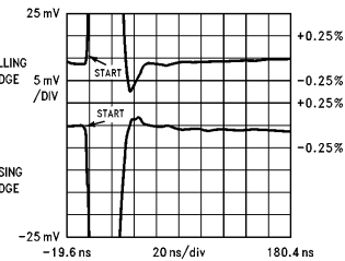
SETTLING RESPONSE V_S = \pm 5\text{V}; R_L = 150\Omega; V_O = \pm 2\text{V}; A_V = -1
