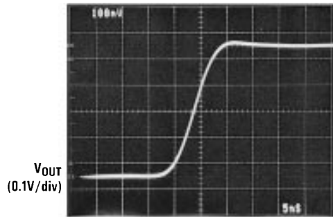
TIME (5 ns/div)
