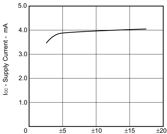
SUPPLY CURRENT
