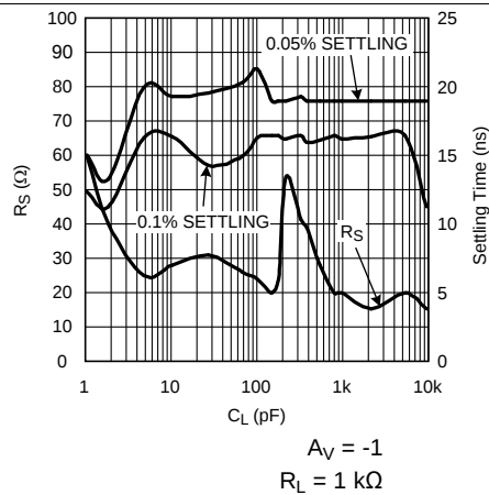
Figure 27. R_S and Settling Time vs. C_L
