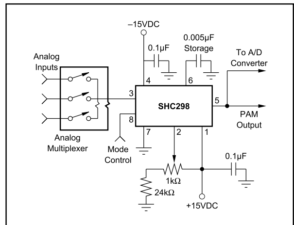
FIGURE 2. Data Acquisition.
