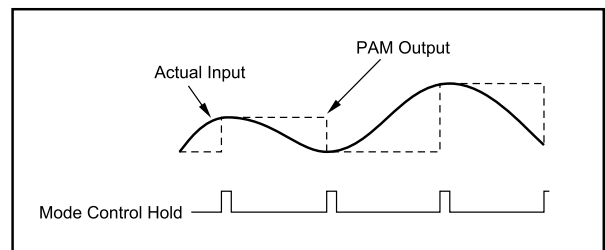
FIGURE 3. PAM Output.
