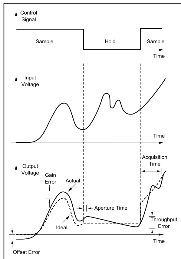
FIGURE 1. Sample/Hold Errors.
