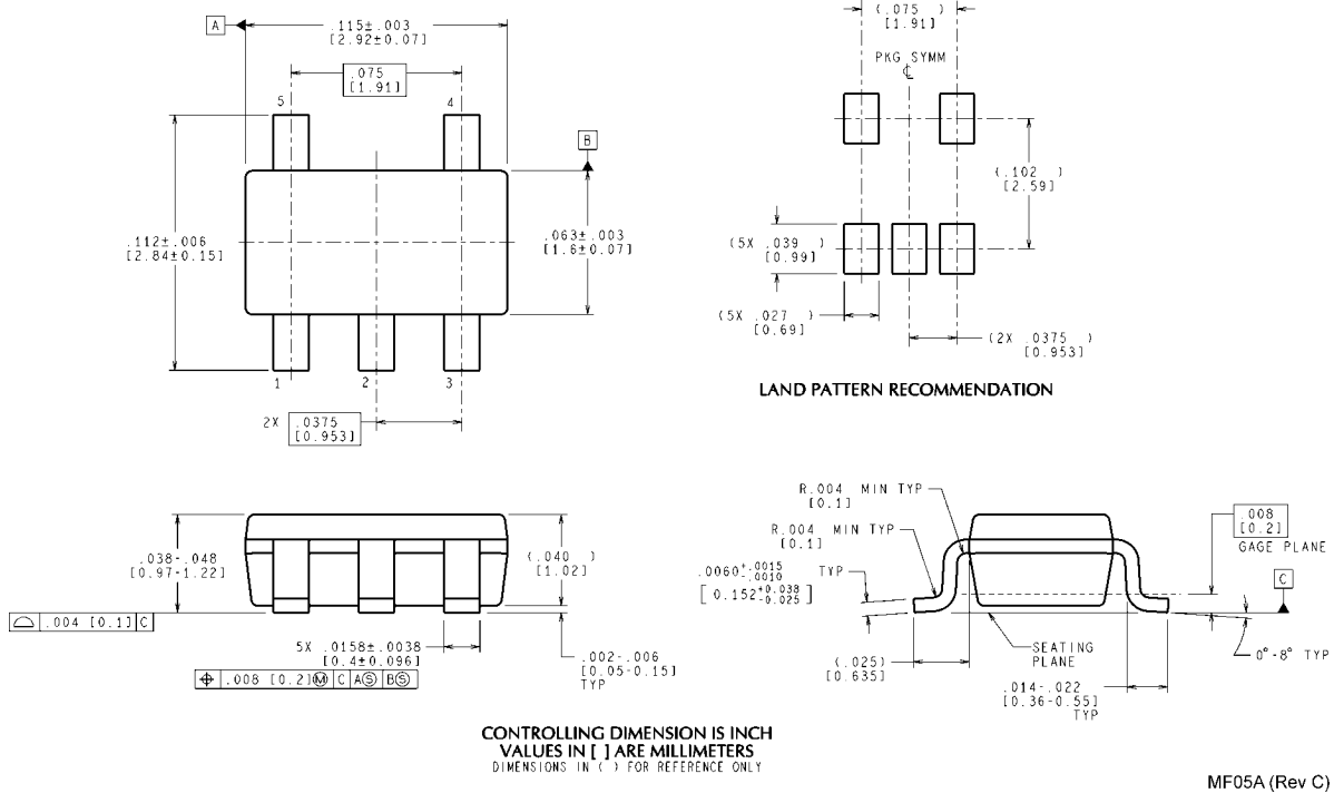
NS Package Number MF05A 5-Lead Small Outline Package SOT23-5 (MF),
