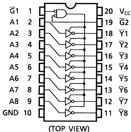
TC74HC540A
