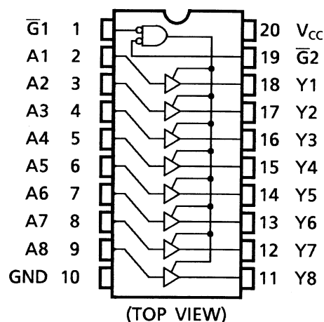
TC74HC541A
