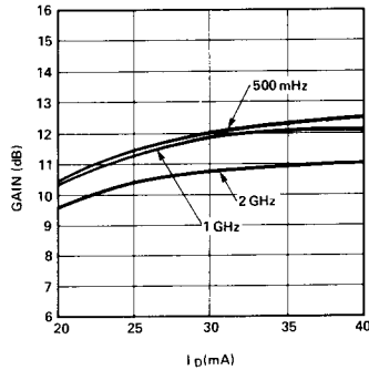
Figure 14. Typical Small Signal Gain vs. I_d at 25°C for the HPMA-0370.
