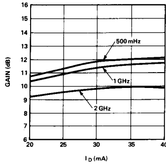
Figure 2. Typical Small Signal Gain vs. I_D at 25°C for the HPMA-0311.
