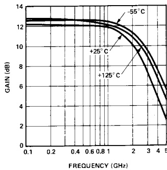
Figure 13. Typical Small Signal Gain vs. Frequency at Three Temperatures for the HPMA-0370.
