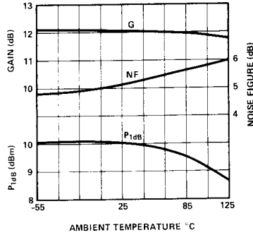
Figure 11. Small Signal Gain, Noise Figure and P_{1dB} vs. Temperature at 1 GHz and I_d = 35 mA for the HPMA-0335.
