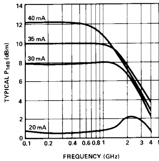
Figure 16. Typical P_{1dB} vs. Frequency at 25°C for the HPMA-0370.
