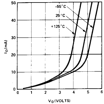
Figure 12. I_d vs. V_d at Three Temperatures for the HPMA-0335.
