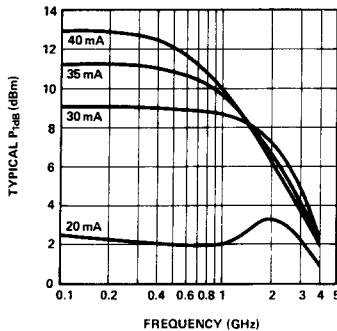
Figure 4. Typical P_{1dB} vs. Frequency at 25°C for the HPMA-0311
