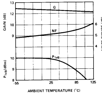
Figure 17. Small Signal Gain, Noise Figure and P_{1dB} vs. Temperature at 1 GHz and I_d = 35 mA for the HPMA-0370.
