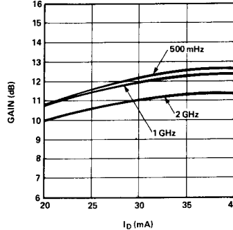
Figure 8. Typical Small Signal Gain vs. I_D at 25°C for the HPMA-0335.
