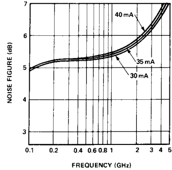
Figure 3. Typical Noise Figure vs. Frequency at 25°C for the HPMA-0311.
