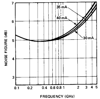
Figure 15. Typical Noise Figure vs. Frequency at 25°C for the HPMA-0370.
