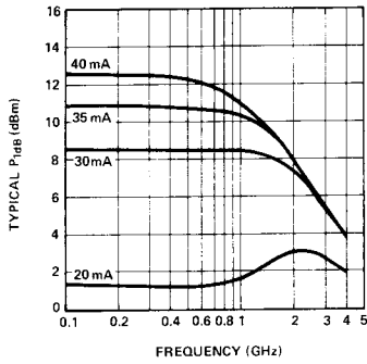
Figure 10. Typical P_{1dB} vs. Frequency at 25°C for the HPMA-0335.
