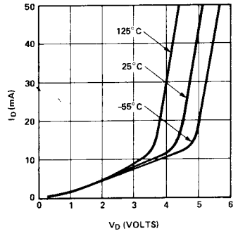
Figure 18. I_d vs. V_d at Three Temperatures for the HPMA-0370.
