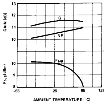
Figure 5. Small Signal Gain, Noise Figure and P_{1dB} vs. Temperature at 1 GHz and I_D = 35 mA for the HPMA-0311.
