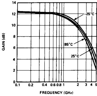
Figure 1. Typical Small Signal Gain vs. Frequency at Three Temperatures for the HPMA-0311.
