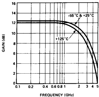
Figure 7. Typical Small Signal Gain vs. Frequency at Three Temperatures for the HPMA-0335.
