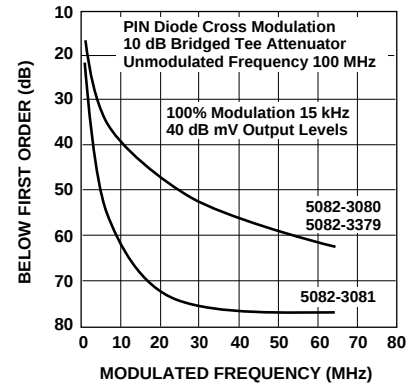
Figure 8. Typical Cross Intermodulation Distortion.
