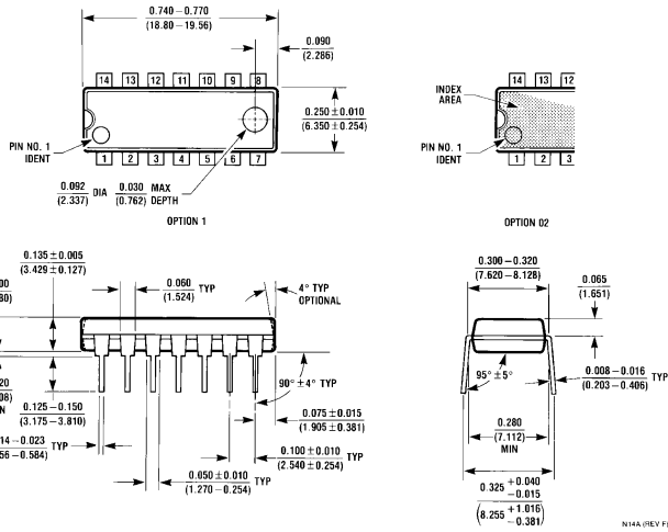
Molded Dual-In-Line Package (N) Order Number LP339N NS Package Number N14A
