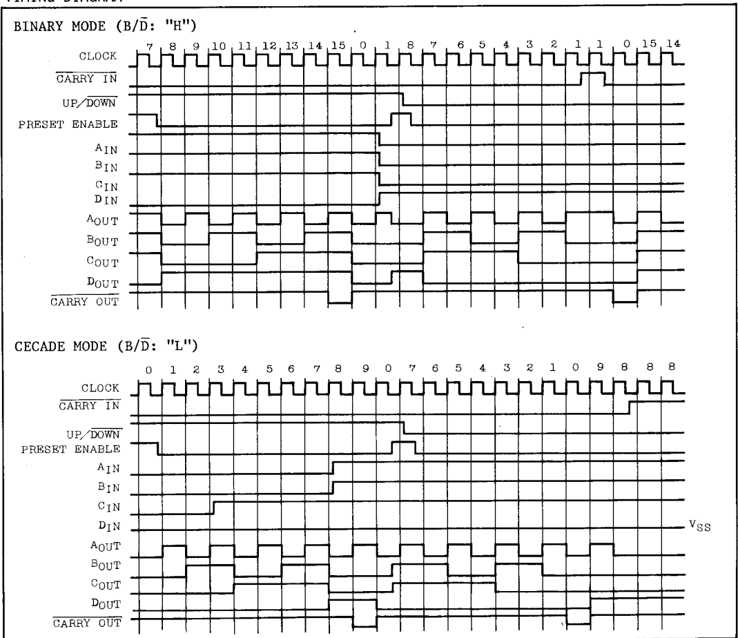
TIMING DIAGRAM
