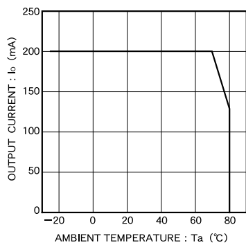
Fig.9 Derating curve
