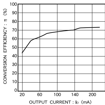
Fig.8 Conversion efficiency
