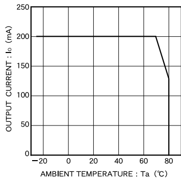
Fig.5 Derating curve
