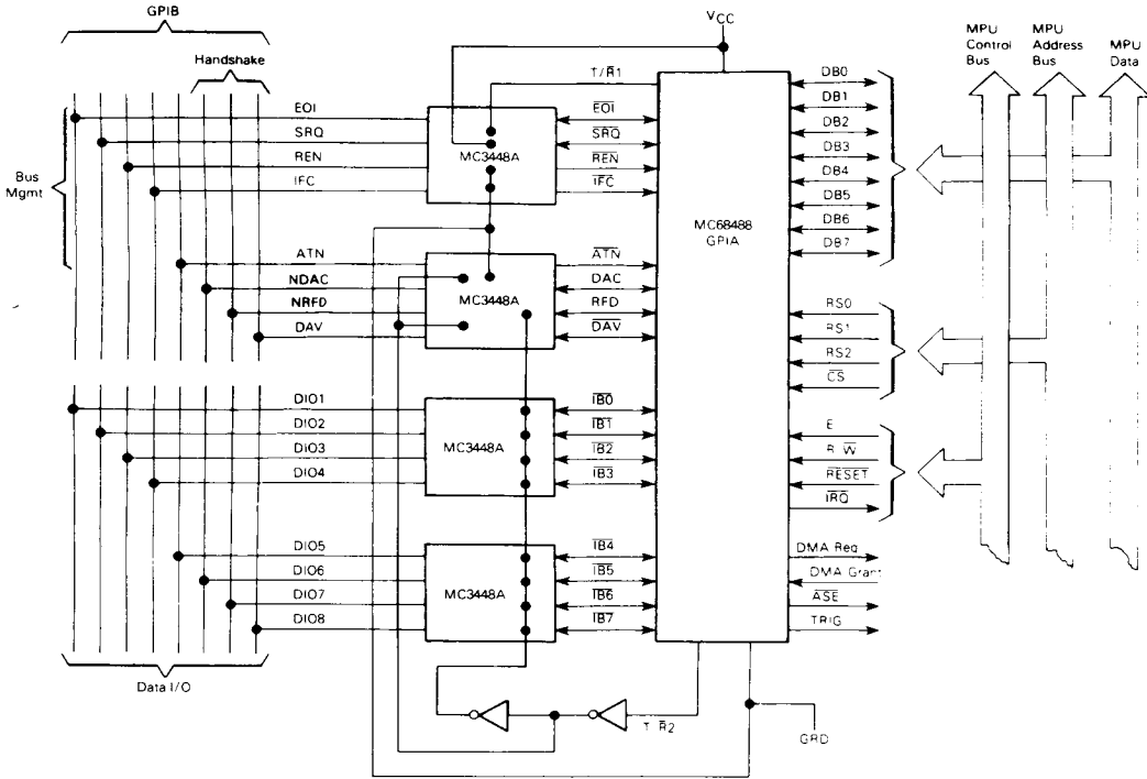
FIGURE 1 — GPIB INTERFACE
