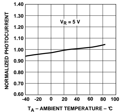
Figure 13. Relative Reverse Light Current vs. Ambient Temperature.
