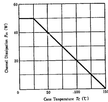
POWER VS. TEMPERATURE DERATING
