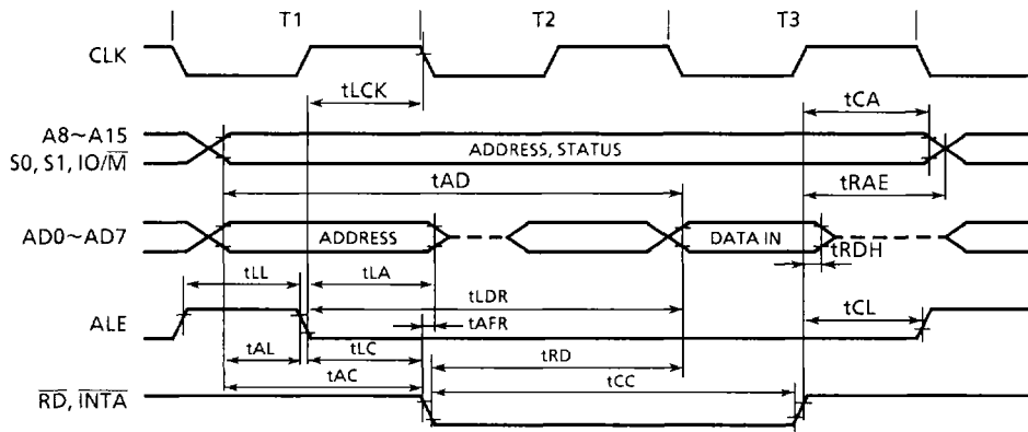
Figure 12.2 Read Operation
