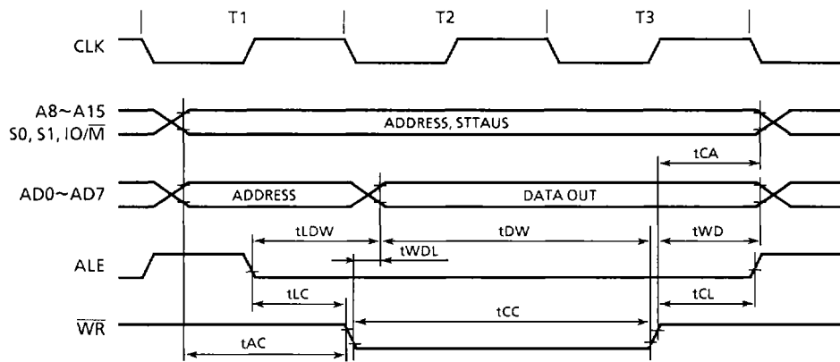
Figure 12.3 Write Operation
