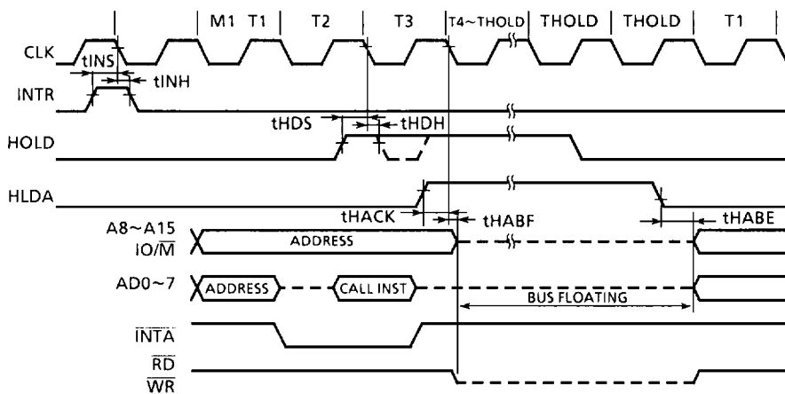
Figure 12.5 Interrupt and Hold Timing
