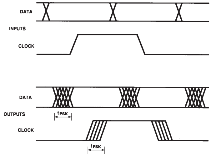
Figure 11. Parallel Data Transmission Example.
