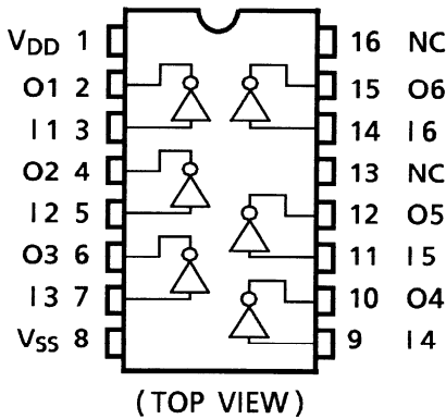
TC4049B
