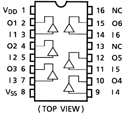
TC4050B
