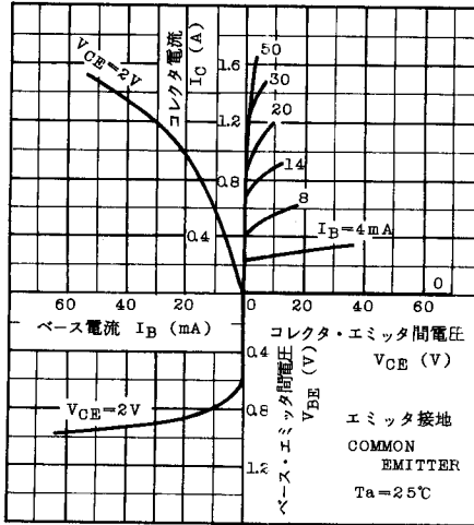
STATIC CHARACTERISTICS
