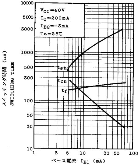
SWITCHING CHARACTERISTICS
